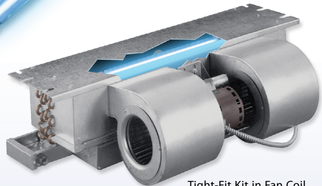
Tight-Fit Kit in Fan Coil
